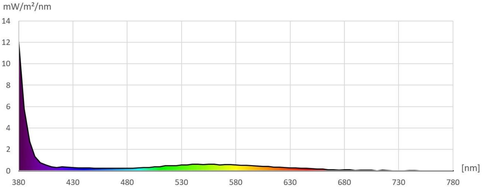
Wavelength UV:
